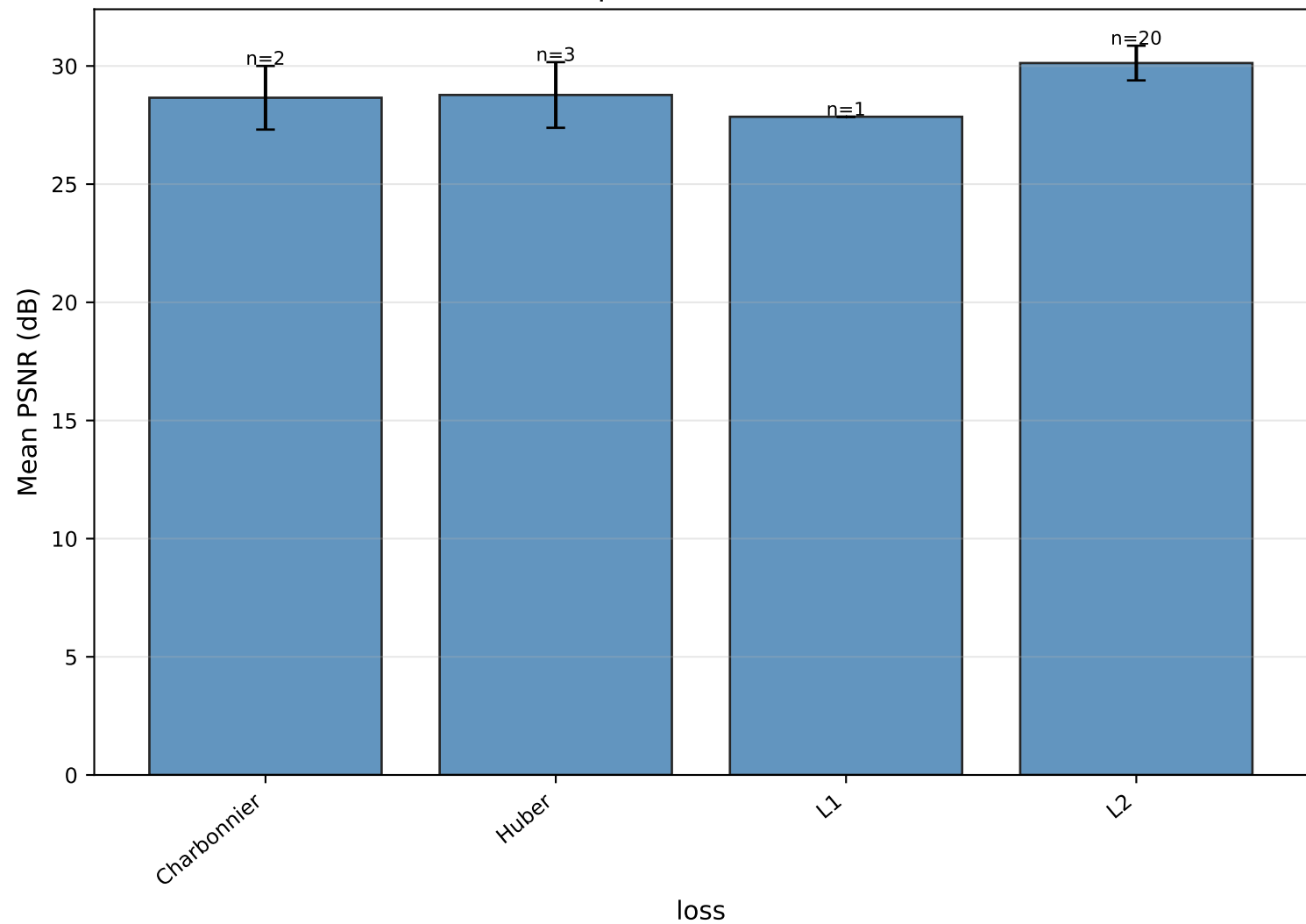
Mean PSNR per value of loss — SwinT
